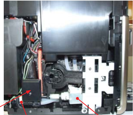
Flow-meter
