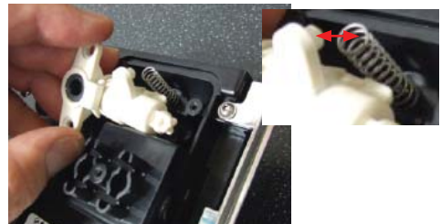
In the reassembling make sure the spring is repositioned correctly (see photo).
